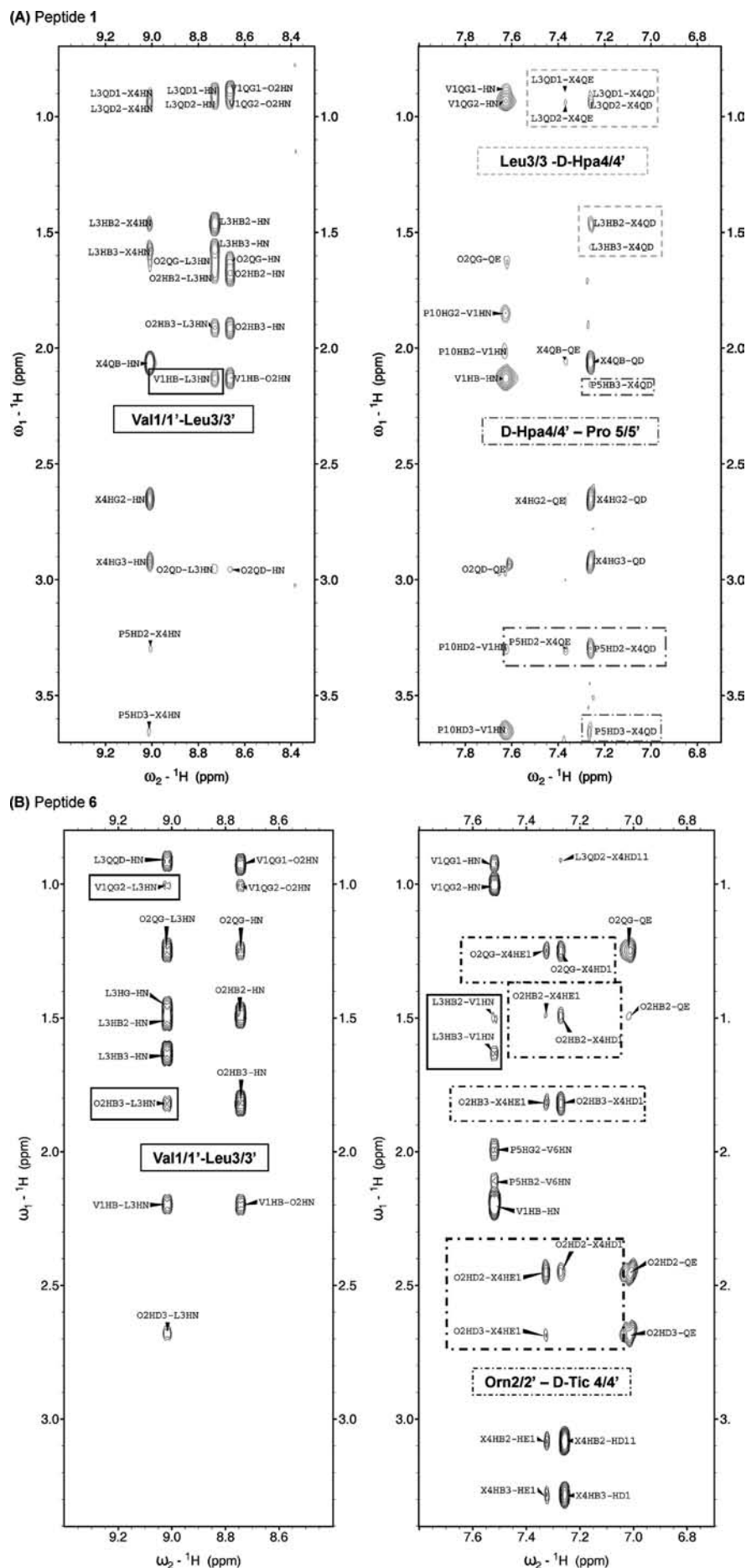
Figure 4. Selected NOESY spectral regions for peptides 1 (A) and 6 (B) in \text{H}_2\text{O}/\text{D}_2\text{O} 9:1 v/v at pH 3 and 5 °C. Relevant sequential and nonsequential NOEs are boxed.
